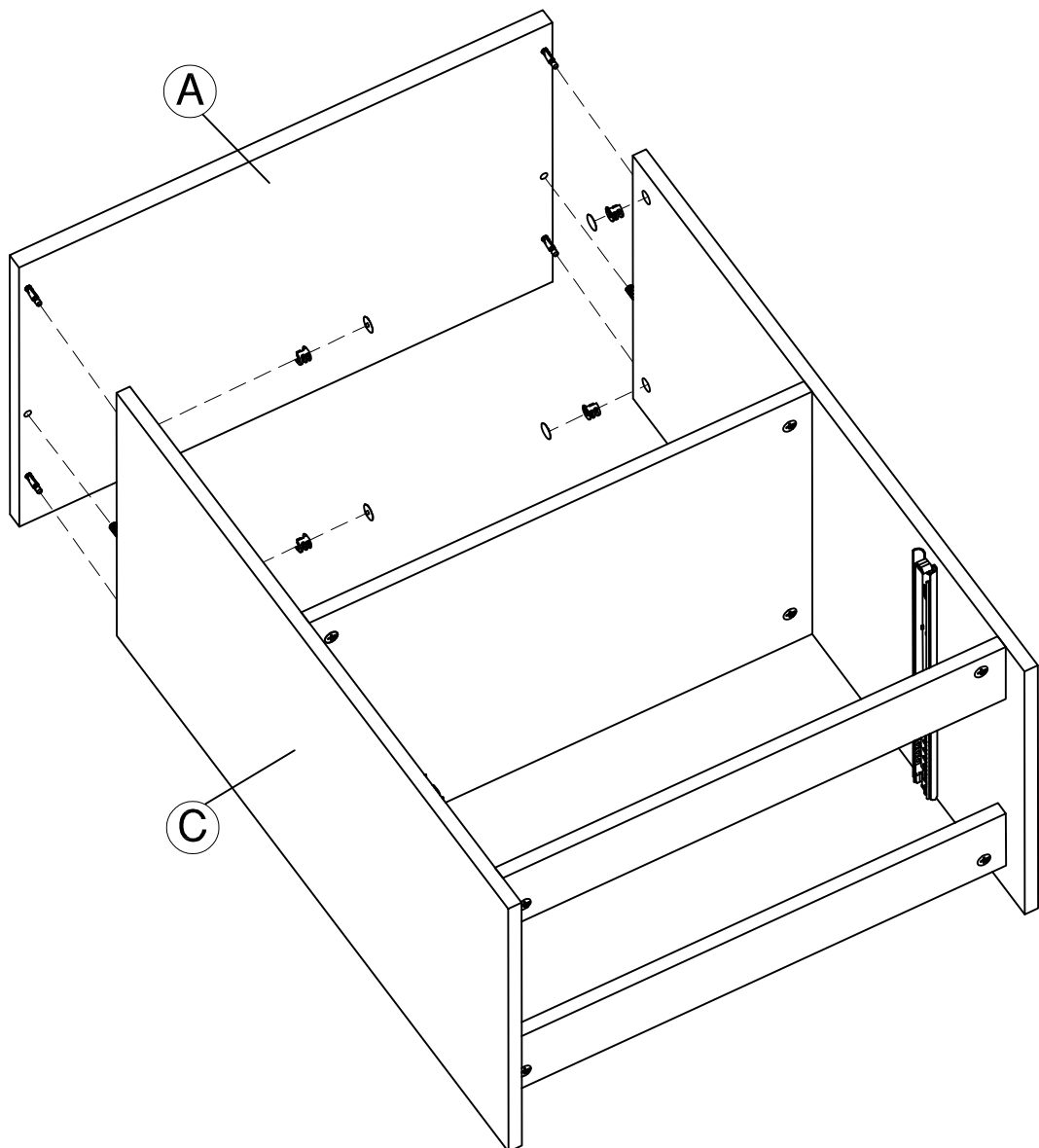
KD Cam
