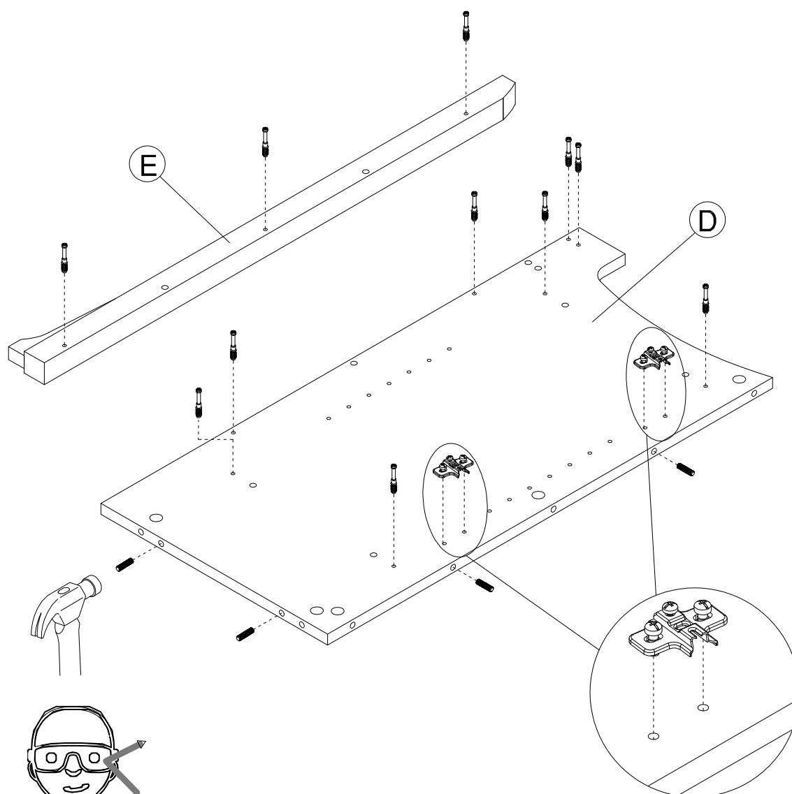
Mounting Plate
